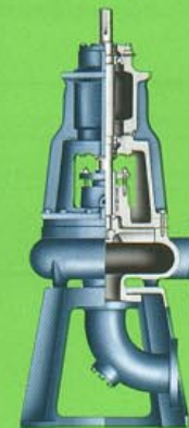
Model HSD Vertical Dry Pit Solids Handling Pump
